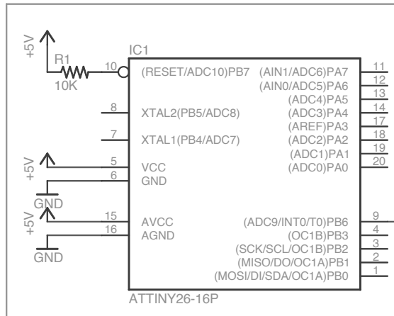
Microcontroller
